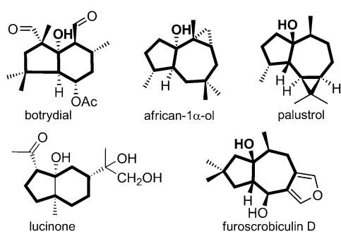
Figure 1. 3a-Hydroxy [n.3.0]carbobicycles in natural products.
