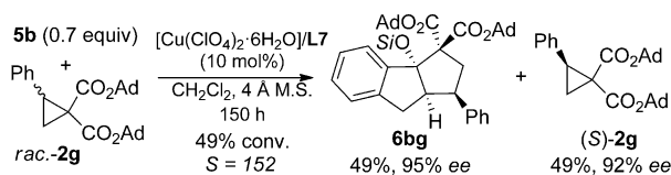
Scheme 2. Concurrent kinetic resolution of the cyclopropane 2g .
